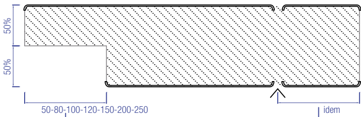
Type 2 Wall with notch and additional saw cut (both sides the same colour, no micro profiling)
